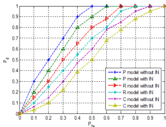
Fig. 7. ROC curve for MMED method with m=8 , SNR = -10 dB
