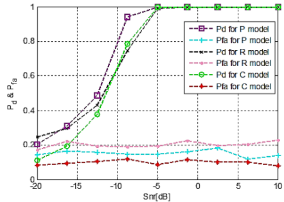
Fig 4. Comparison of Pd, Pfa Vs SNR
