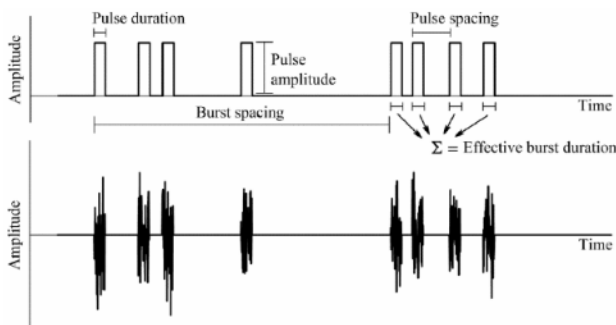
Fig. 2. Waveform for Impulsive Noise.
