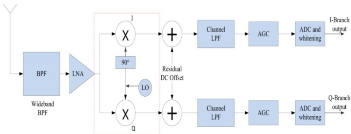
Fig.1. CR Receiver diagram
