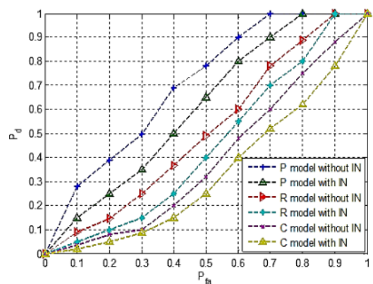
Fig.5. ROC curve for ED method with m=8 , SNR = -10 dB.
