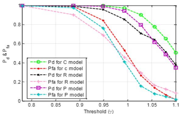
Fig. 3. Pd, Pfa Vs Threshold
