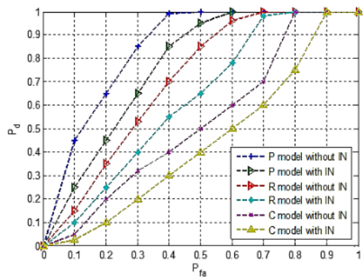
Fig. 6. ROC curve for GLRT method with m=8 , SNR = -10 dB.
